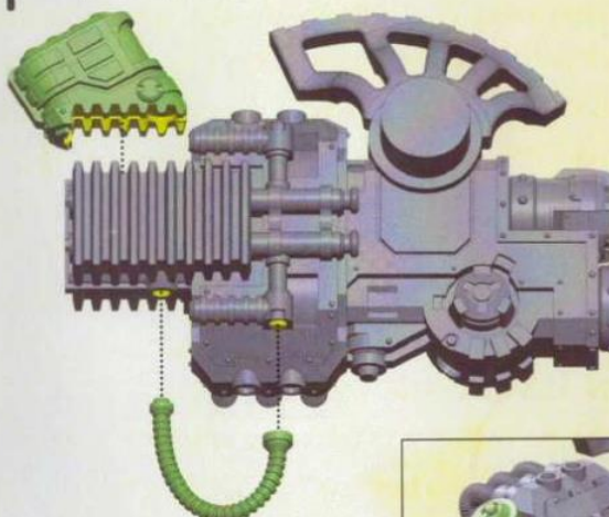
72. Power Cable
