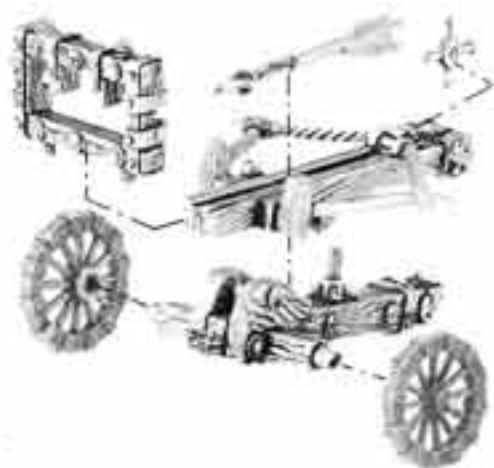
BOLT THROWER BOLT 020504207
